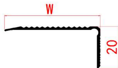
图纸和尺寸Drawing and dimensions:
