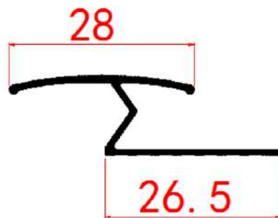
图纸和尺寸Drawing and dimensions:
