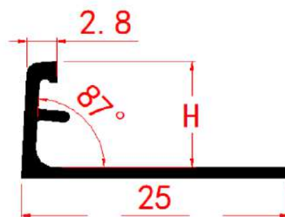
图纸和尺寸Drawing and dimensions:
