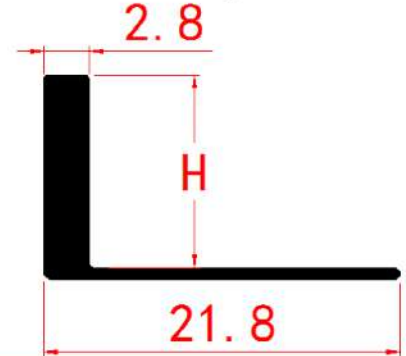
图纸和尺寸Drawing and dimensions:
