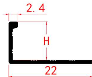
图纸和尺寸Drawing and dimensions:
