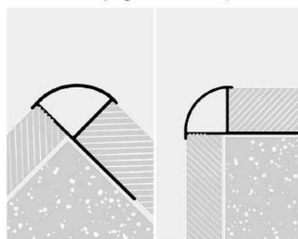
铺设方法示例Laying method example:
