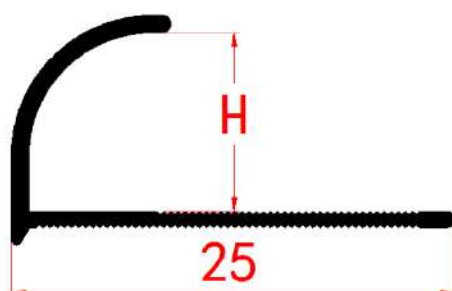
图纸和尺寸Drawing and dimensions:
