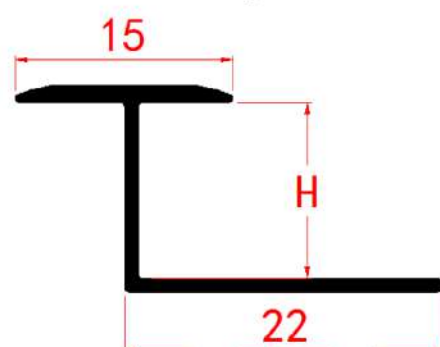
图纸和尺寸Drawing and dimensions:
