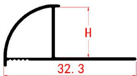
图纸和尺寸Drawing and dimensions:
