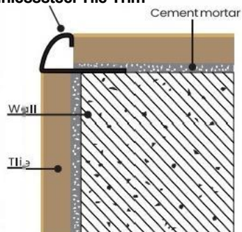
stainlesssteel Tile Trim
